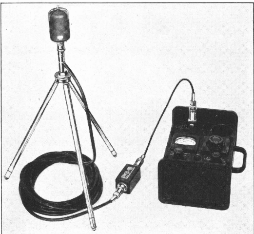
(B) Microphone and transformer plug into the sound-level meter as shown above.
