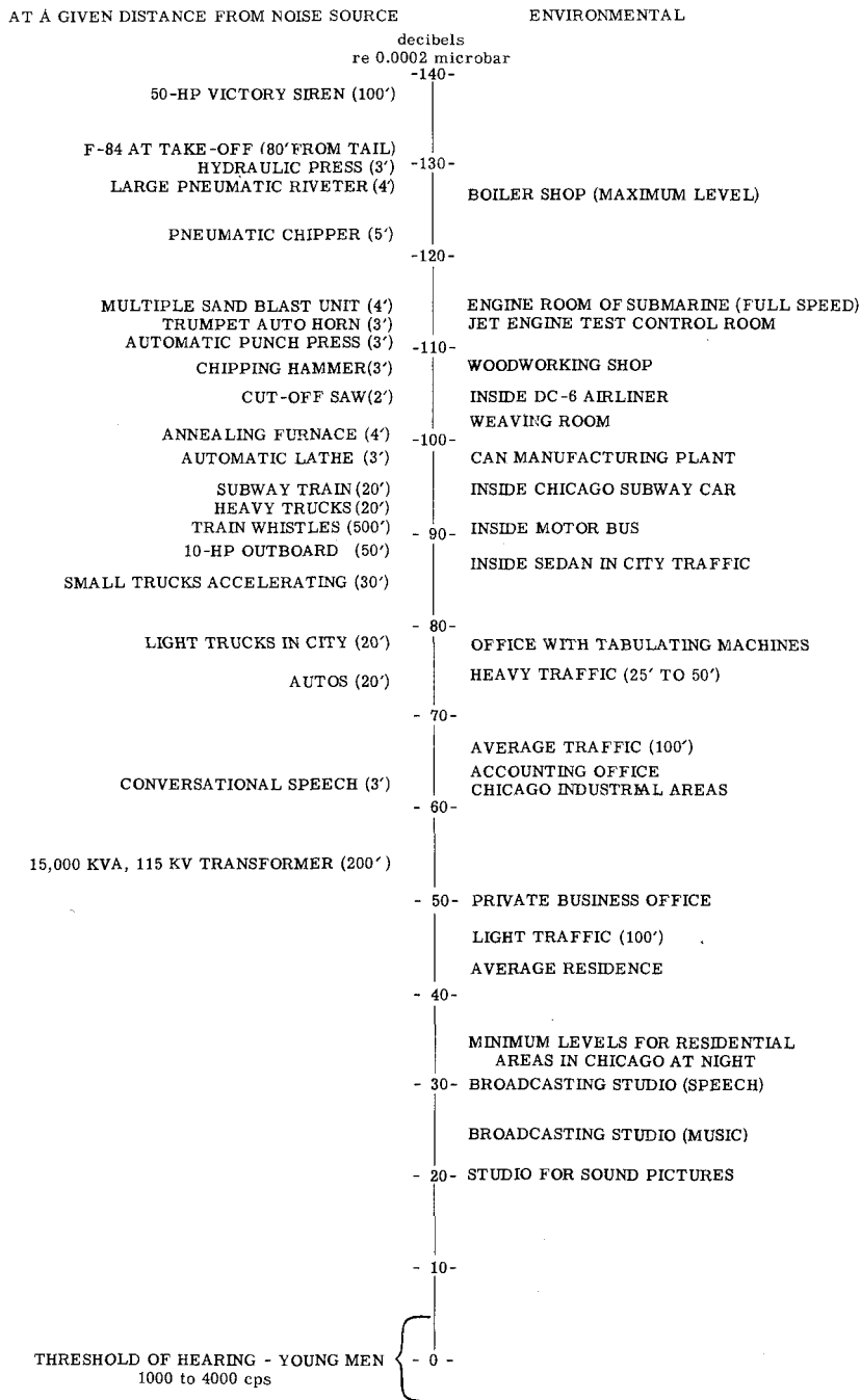
Figure 2-1. Typical over-all sound levels measured with a sound-level meter (levels below 85 db are weighted according to the method given in Section 2.3). Sound-level measurements give only part of the information usually necessary to handle noise problems and are often supplemented by analysis of the noise spectra and by oscillographic studies.
