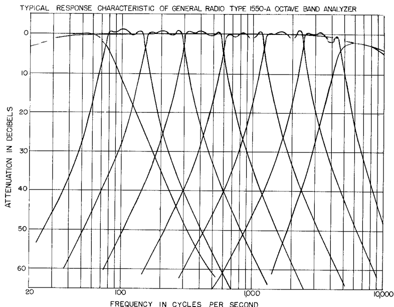
Figure 6-4. Typical response characteristics of the Type 1550-A Octave-Band Noise Analyzer.
