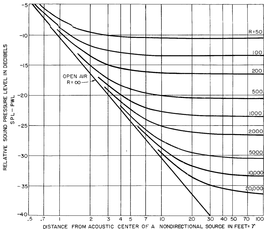
Figure 8-3. Chart showing the sound-pressure level, SPL, relative to the power level, PWL, for a non-directional source for different values of the room constant, R , as a function of the distance from the source.
