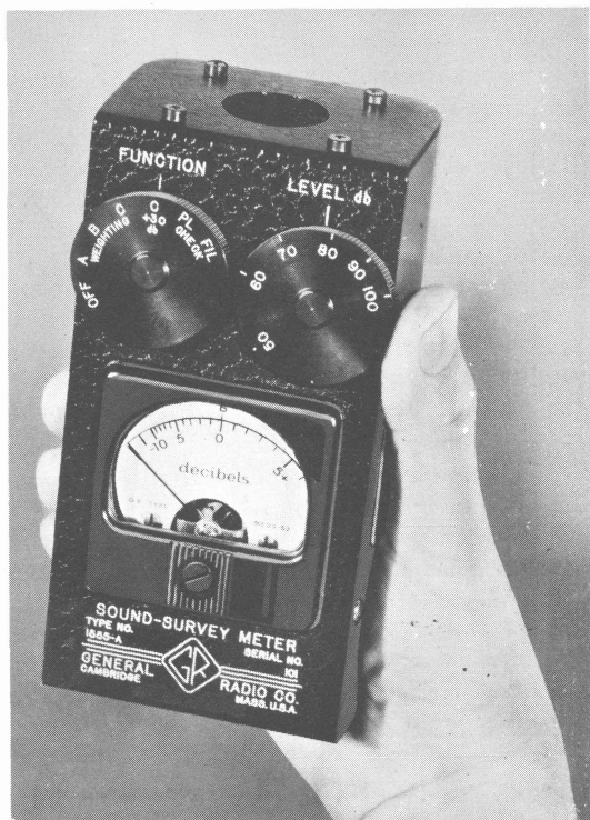
Figure 4-2. The Type 1555-A Sound-Survey Meter.
