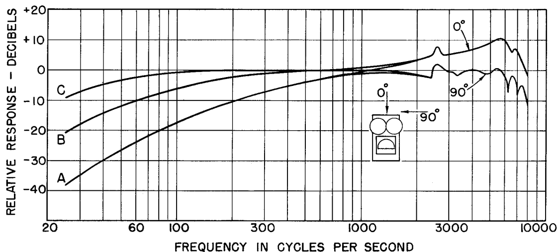
Figure 6-2. Typical over-all free-field response characteristics of the Type 1555-A Sound-Survey Meter.
