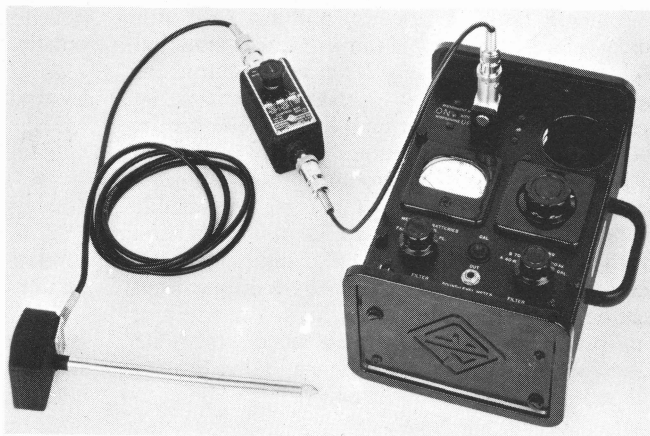
Figure 6-15. The Type 759-P35 Vibration Pickup and Type 759-P36 Control Box used with the Type 1551-A Sound-Level Meter.
