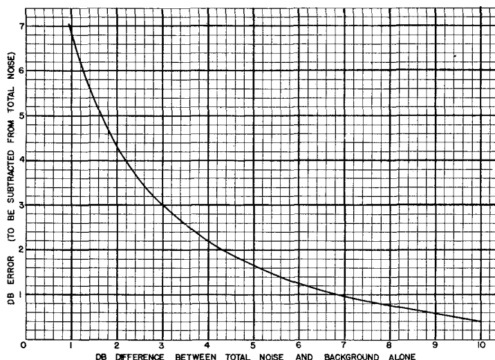
Figure 6-13. Background noise correction for sound-level measurements.
