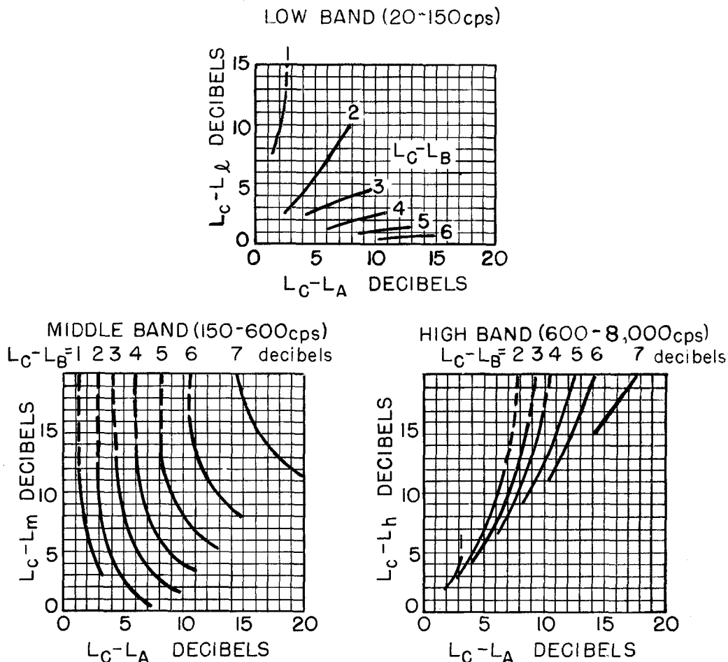
Figure 6-3. Curves for calculating an approximate frequency analysis in three bands from level readings taken when using the three sound-level meter weighting networks. The measured value of L_C - L_A is entered at the abscissa of each graph, proceeding vertically to the curve labeled with the measured value of L_C - L_B , then horizontally to the ordinate value for each of the three bands corresponding to the difference between the individual band levels and the over-all level. (This method of analysis was developed by J. R. Cox, Liberty Mutual Insurance Company.)
