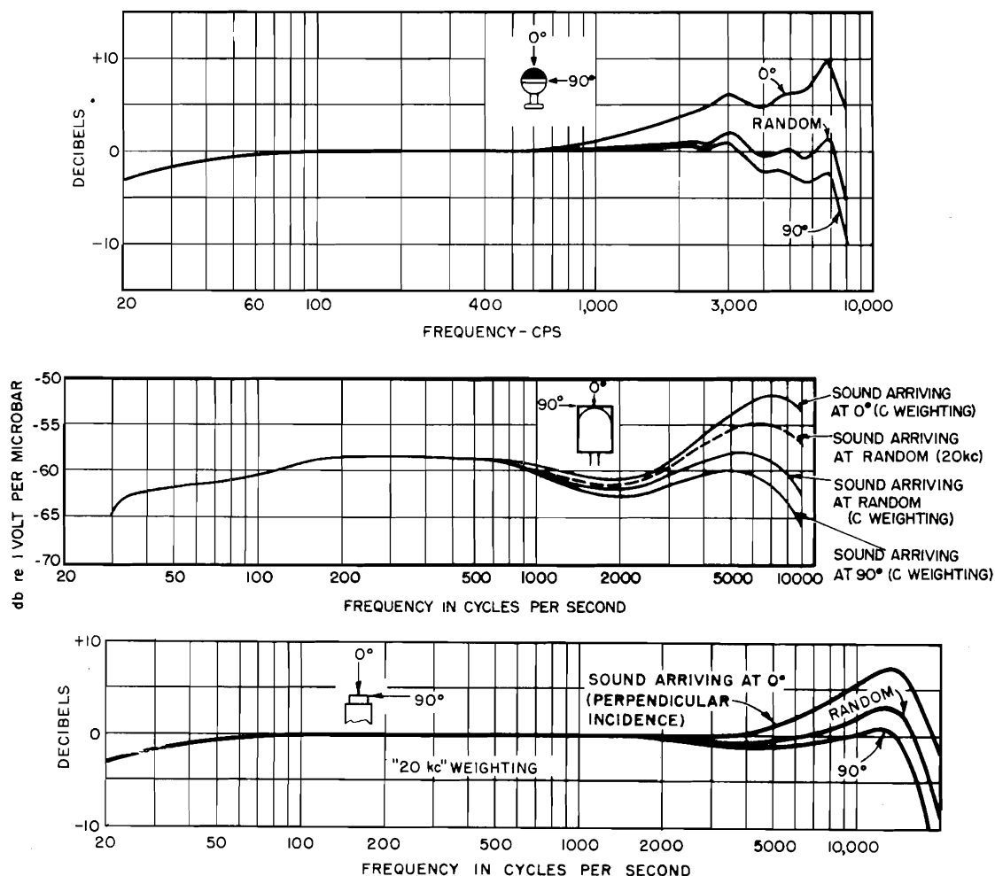
Figure 6-10. Typical response curves for three different microphones when used with the Type 1551-A Sound-Level Meter. (From top to bottom) (a) Rochelle-salt crystal microphone normally supplied with the Type 1551-A; (b) the Type 759-P25 Dynamic Microphone; and (c) the Type 1551-P1 Condenser Microphone. Random response assumes that the microphone is placed in a diffuse sound field.
