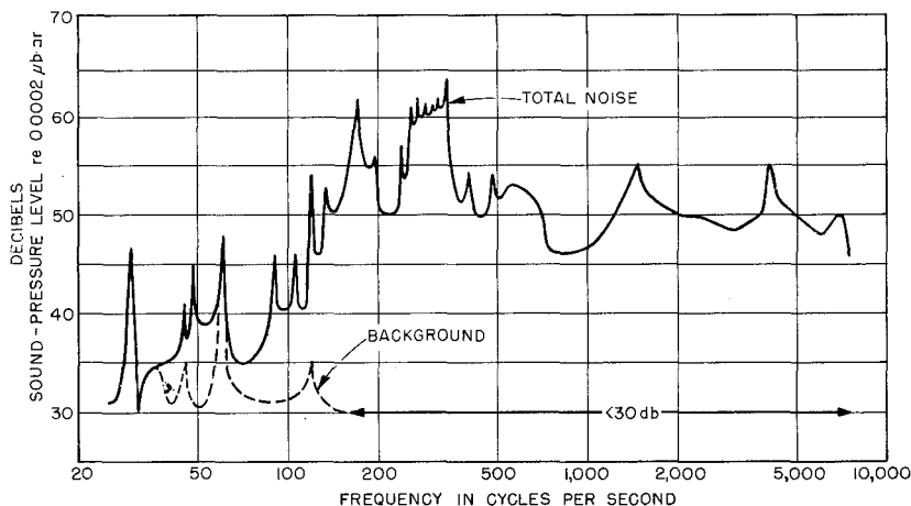
Figure 6-7. A plot of the noise analysis made with a Type 760-B Ana- lyzer on the same machine as in Figure 6-5.
