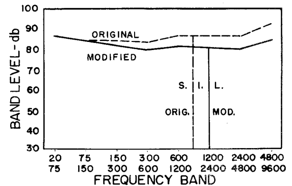
Figures 9-1 to 9-4. Examples to illustrate the possible noise reduction effects of some noise control measures.
