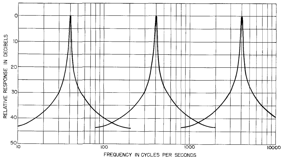
Figure 6-6. Typical response characteristics of the Type 760-B Sound Analyzer for three representative frequency settings.
