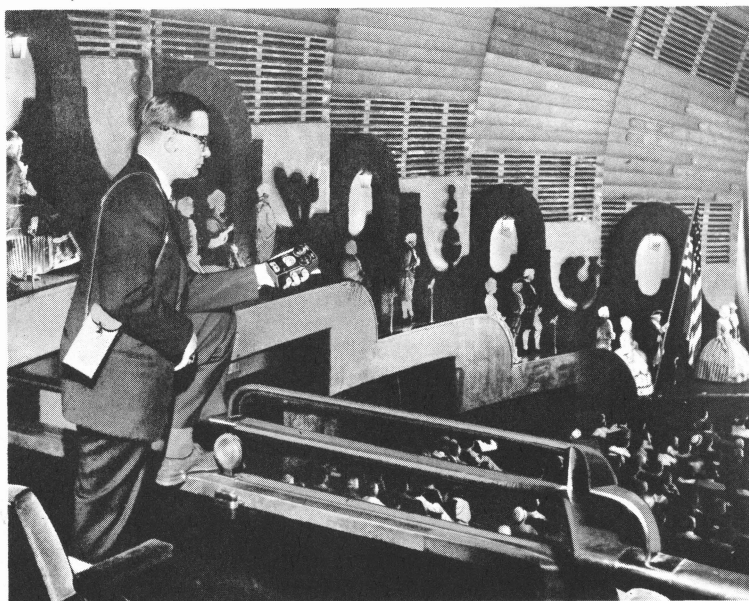
Figure 5-3. Performance checks of sound reinforcement system at Radio City Music Hall being made with Sound-Survey Meter.
