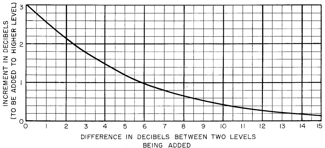
Figure 2-4. Chart for combining noise levels.
