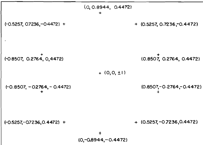
Figure 8-7. Plan view of twelve points uniformly distributed on a sphere of unit radius. Coordinates are given as in the previous figure. When measurements are to be made on a hemisphere, only the six points above the x - y reference plane (positive values of z ) are used.
