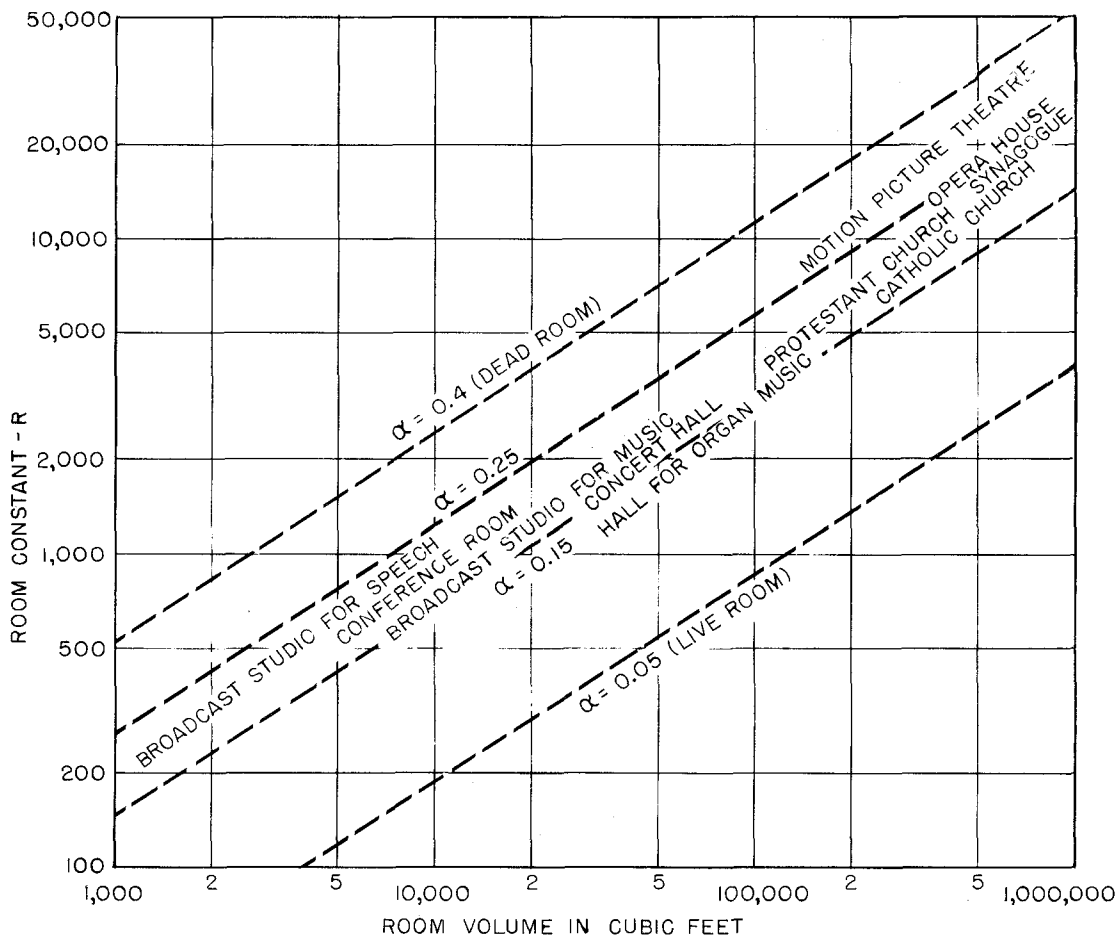
Figure 8-5. The relation between the room constant, R , and the volume of the room for four different values of the average absorption, \alpha , in the room. For purposes of comparison, representative values of R for rooms used for various purposes are also shown. These values are indicated by placing the name at the level generally regarded as optimum acoustically for that class of service. Thus a broadcast studio used for music is usually designed to have a room constant of about 400 if it is as small as 5000 cubic feet or a room constant of about 5000 if it is as large as 100,000 cubic feet.
