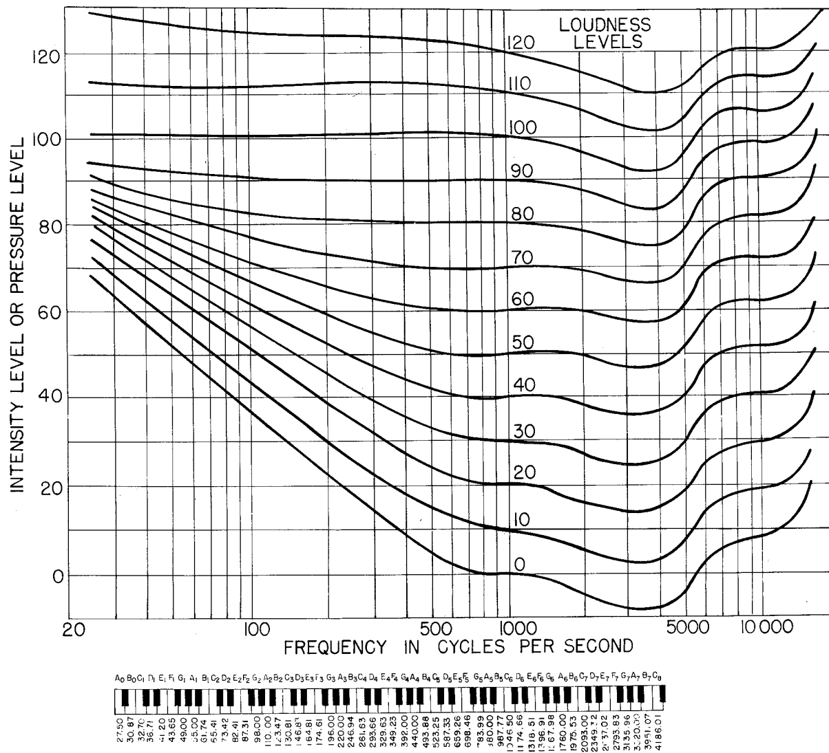
Figure 3-3. Free field equal-loudness contours of pure tones (Fletcher-Munson curves). Piano keyboard helps identify the frequency scale. Only the fundamental frequency of each piano key is indicated.
