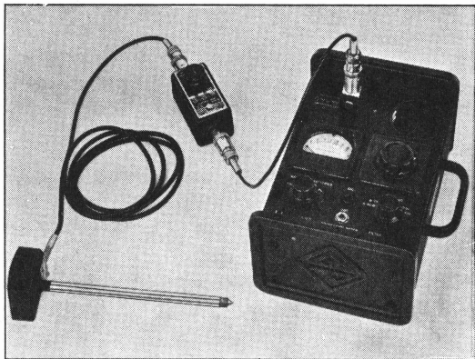
The vibration pickup and control box plug into the sound-level meter in place of the microphone, as shown in the photograph above.
