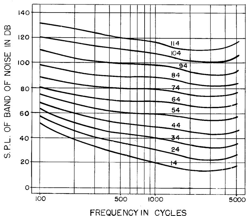
Figure 3-4. Equal-loudness contours for relatively narrow bands of random noise. The center frequency of the band is shown as the abscissa, and the numbers on the curves are phons. (Irwin Pollack, "The Loudness of Bands of Noise," Jour. Acoust. Soc. Am. , Vol. 24, Sept., 1952, pp. 533-538)
